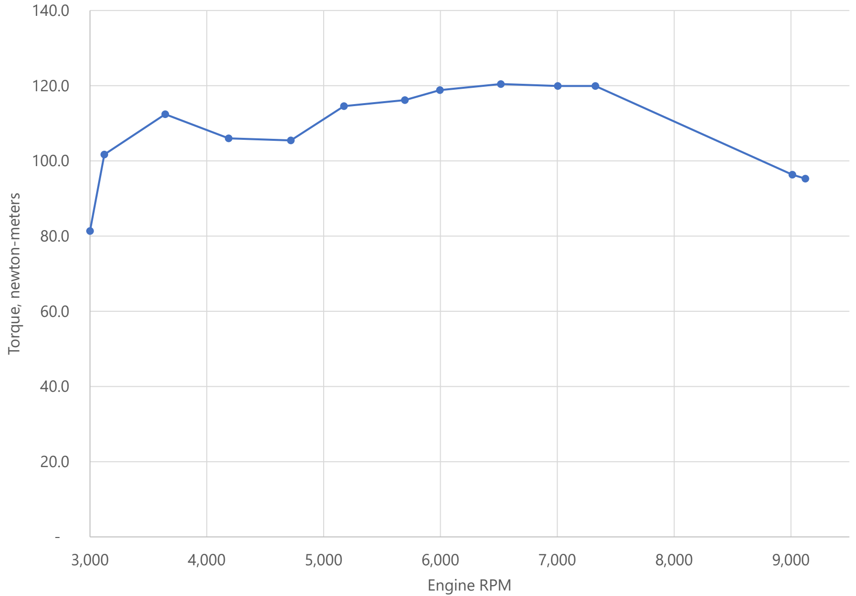
Engine Torque vs RPM
